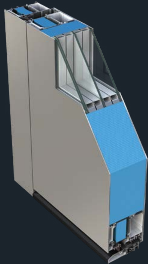
S-200 FLAT CROSS SECTION
